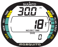
Fig. 3.9. Planning. The no-decompression time limit at 30.0 m [100 ft] is 18 minutes in PO/A0 mode..
