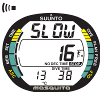
Fig. 3.15 Ascent Rate Indicator. Blinking SLOW and four segments are shown together with an audible alarm: ascent rate is more than 10 m/min [33 ft/min]. This is a caution to slow down! STOP sign means that you are advised to make a Mandatory Safety Stop when you reach a depth of 6
